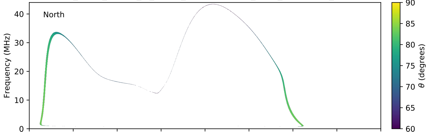
expres_earth_jupiter_io_jrm09_lossc-wid1deg_3kev_20041222_v11.cdf
