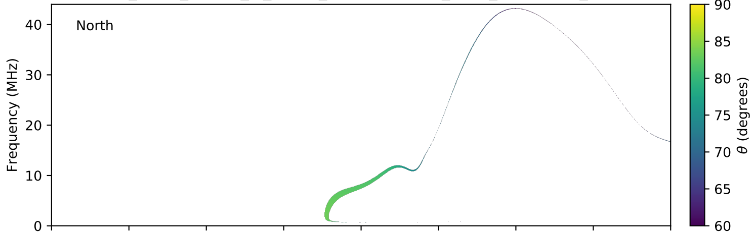
expres_earth_jupiter_io_jrm09_lossc-wid1deg_3kev_20041218_v11.cdf
