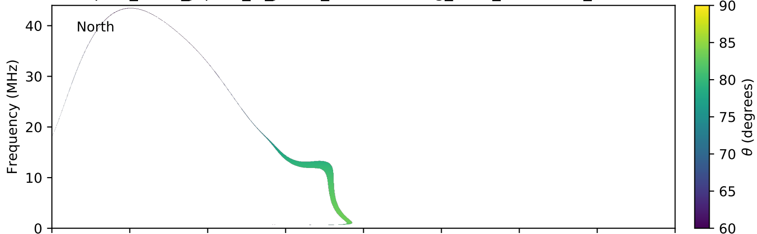
expres_earth_jupiter_io_jrm09_lossc-wid1deg_3kev_20041217_v11.cdf
