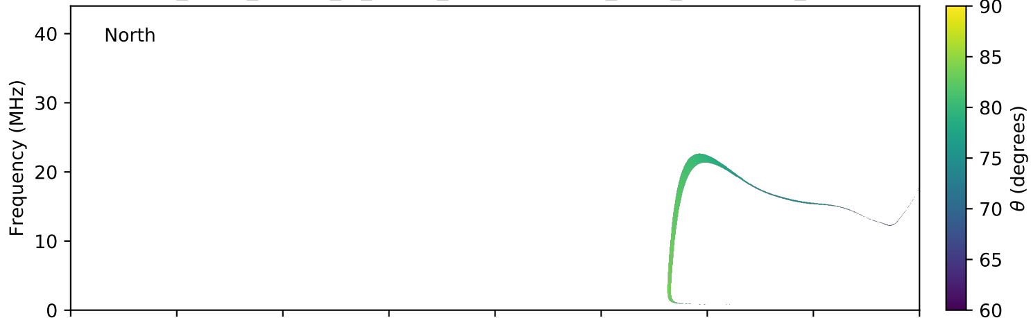
expres_earth_jupiter_io_jrm09_lossc-wid1deg_3kev_20041216_v11.cdf
