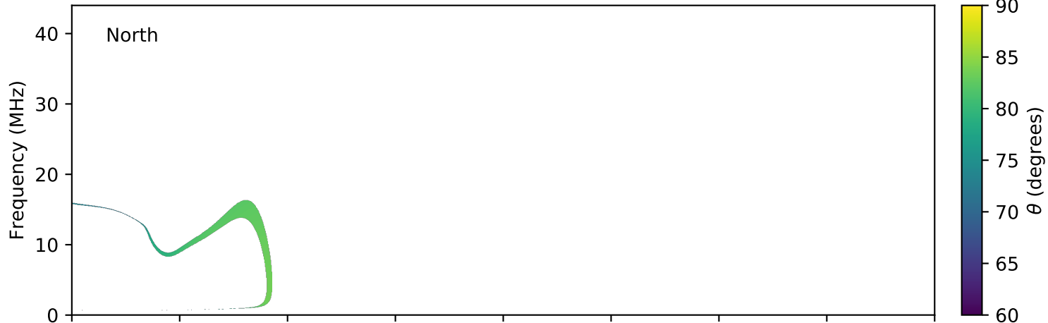
expres_earth_jupiter_io_jrm09_lossc-wid1deg_3kev_20041212_v11.cdf
