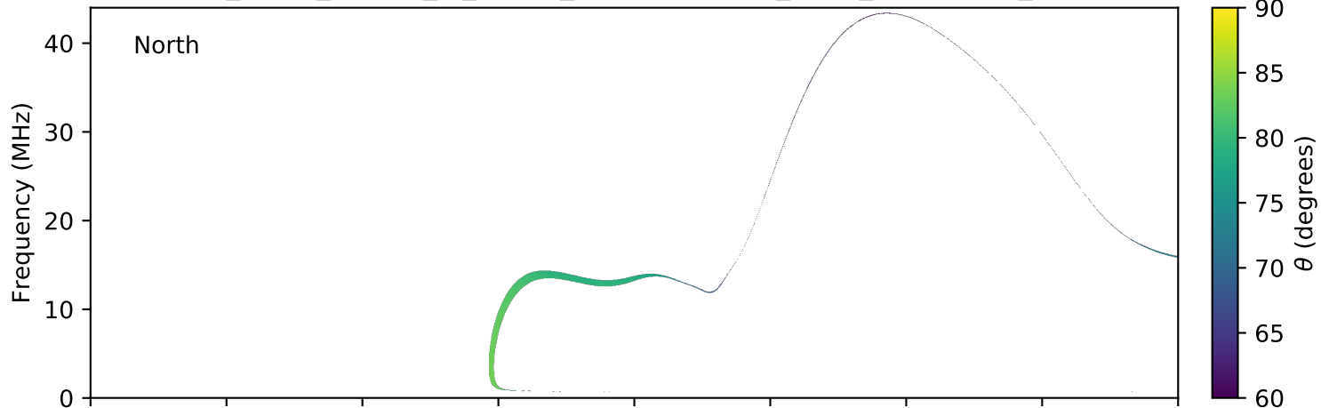
expres_earth_jupiter_io_jrm09_lossc-wid1deg_3kev_20041211_v11.cdf
