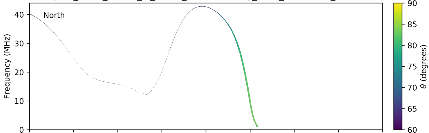
expres_earth_jupiter_io_jrm09_lossc-wid1deg_3kev_20041208_v11.cdf
