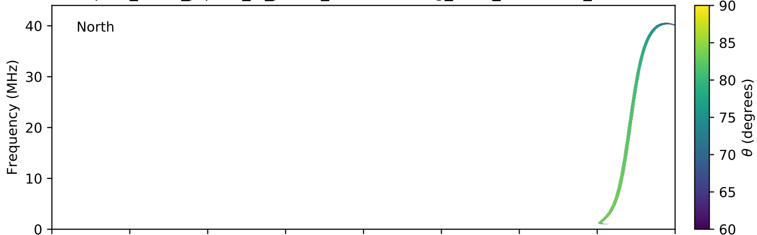
expres_earth_jupiter_io_jrm09_lossc-wid1deg_3kev_20041207_v11.cdf
