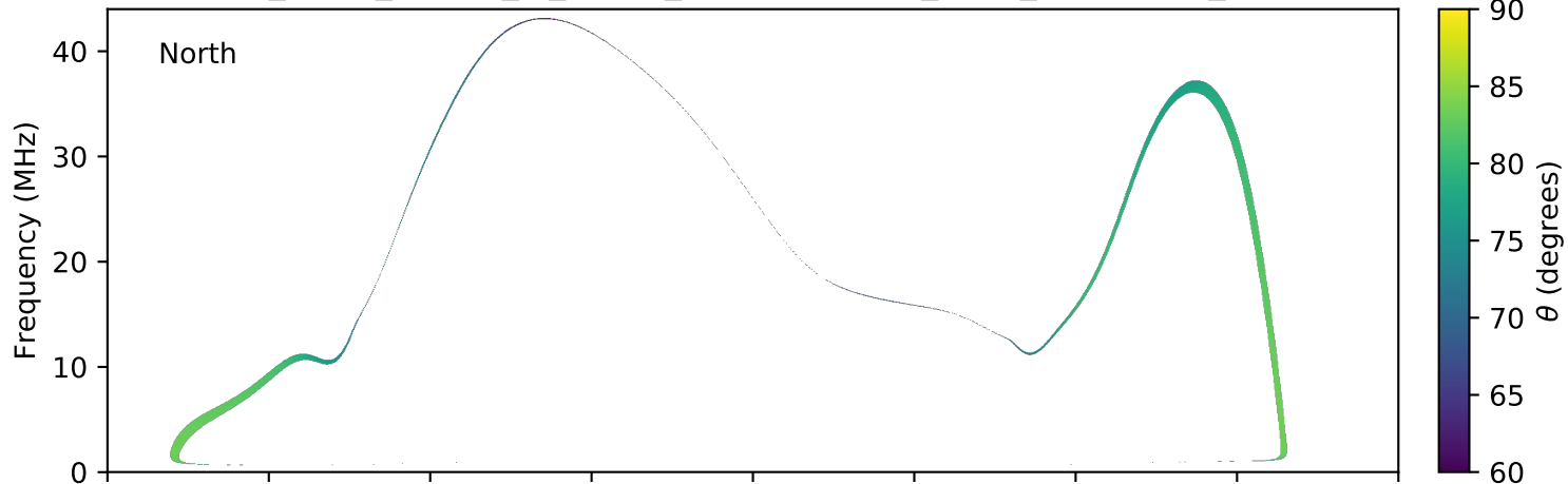
expres_earth_jupiter_io_jrm09_lossc-wid1deg_3kev_20041206_v11.cdf
