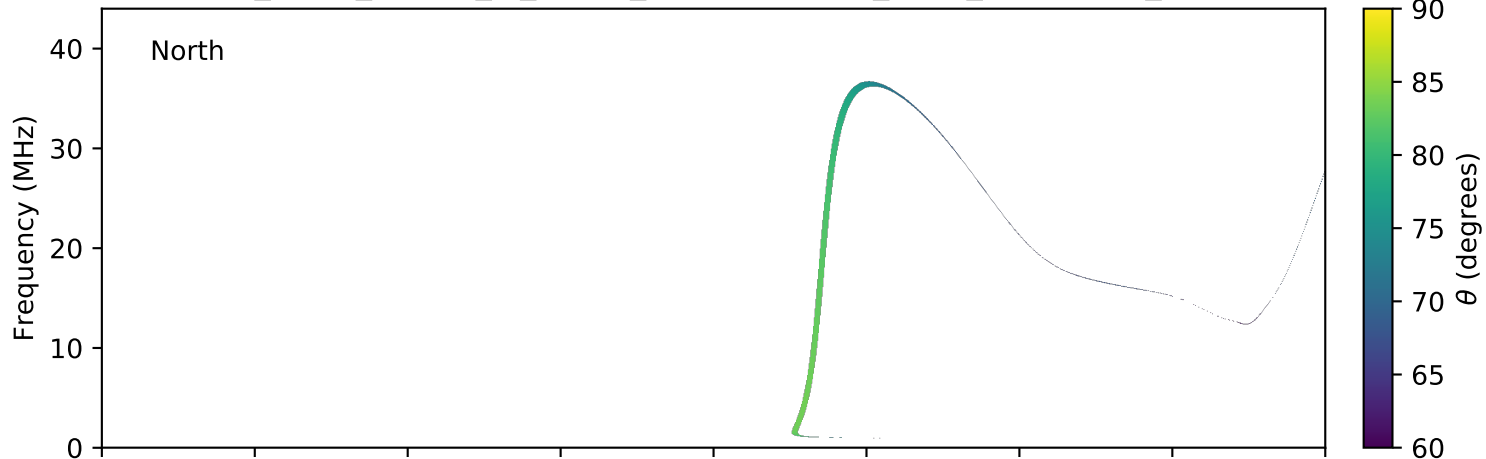
expres_earth_jupiter_io_jrm09_lossc-wid1deg_3kev_20041202_v11.cdf
