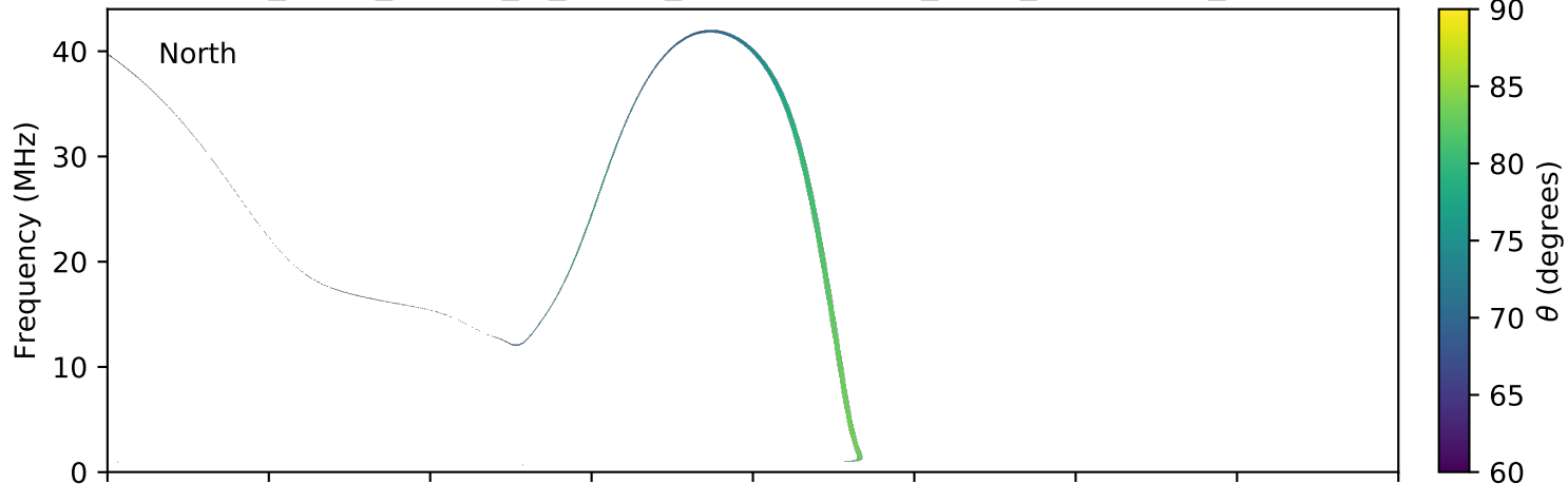
expres_earth_jupiter_io_jrm09_lossc-wid1deg_3kev_20041201_v11.cdf
