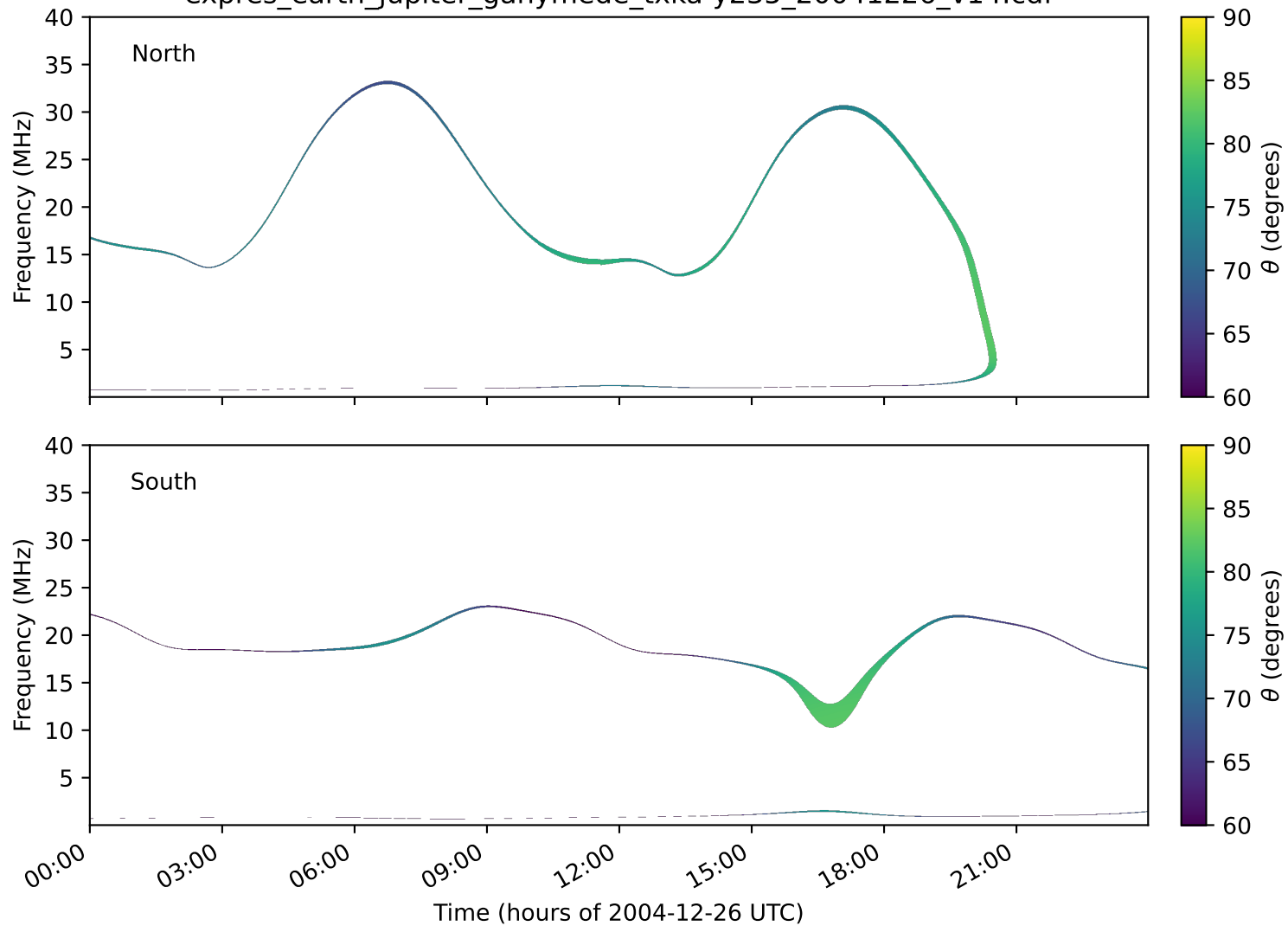
expres_earth_jupiter_ganymede_txka-y235_20041226_v14.cdf
