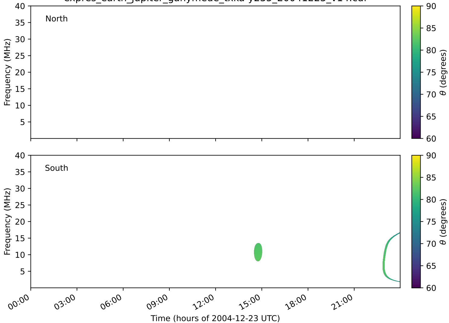
expres_earth_jupiter_ganymede_txka-y235_20041223_v14.cdf
