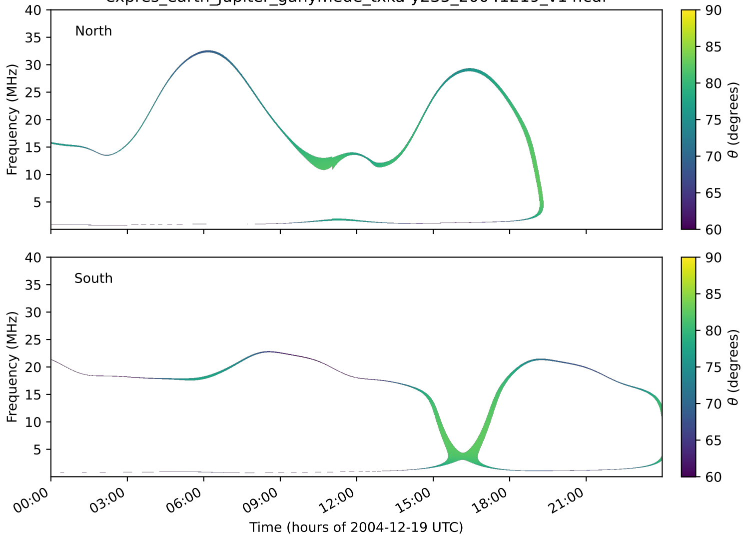
expres_earth_jupiter_ganymede_txka-y235_20041219_v14.cdf
