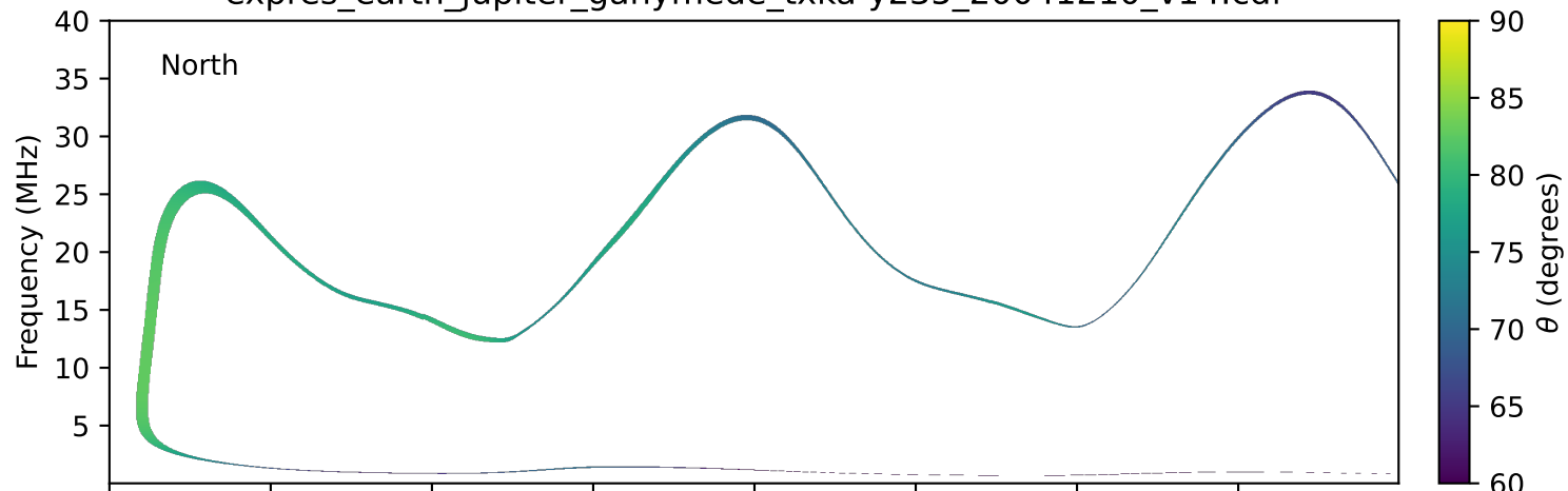
expres_earth_jupiter_ganymede_txka-y235_20041210_v14.cdf
