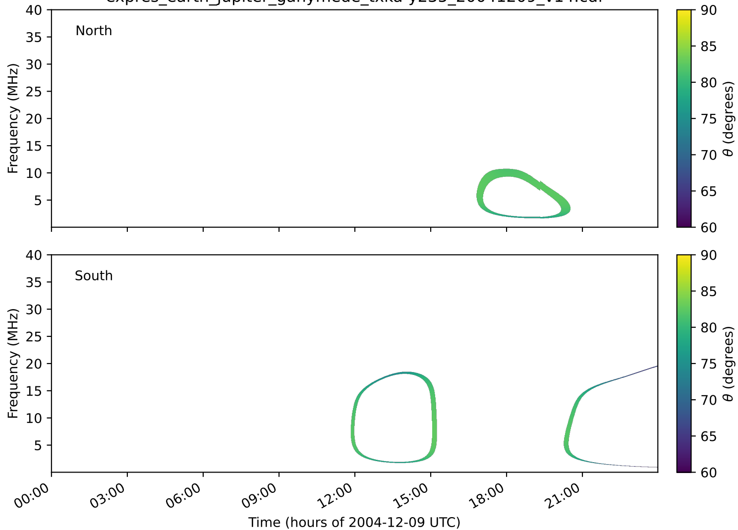
expres_earth_jupiter_ganymede_txka-y235_20041209_v14.cdf
