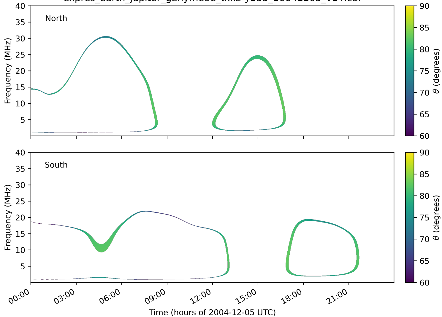
expres_earth_jupiter_ganymede_txka-y235_20041205_v14.cdf
