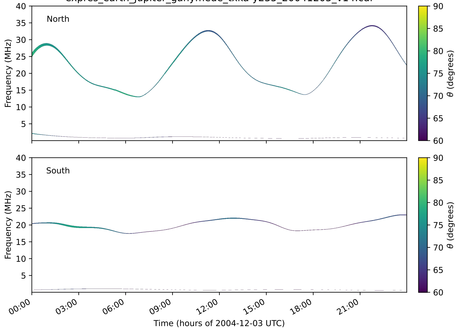
expres_earth_jupiter_ganymede_txka-y235_20041203_v14.cdf
