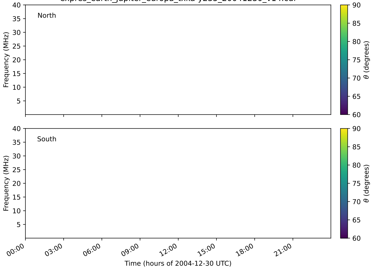
expres_earth_jupiter_europa_txka-y235_20041230_v14.cdf
