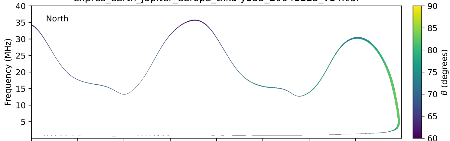
expres_earth_jupiter_europa_txka-y235_20041225_v14.cdf
