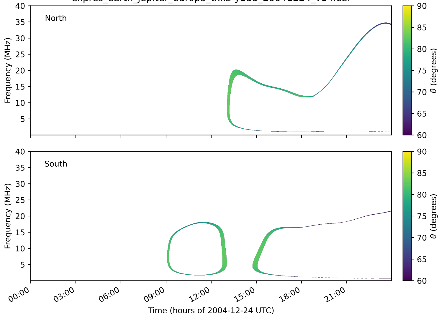
expres_earth_jupiter_europa_txka-y235_20041224_v14.cdf
