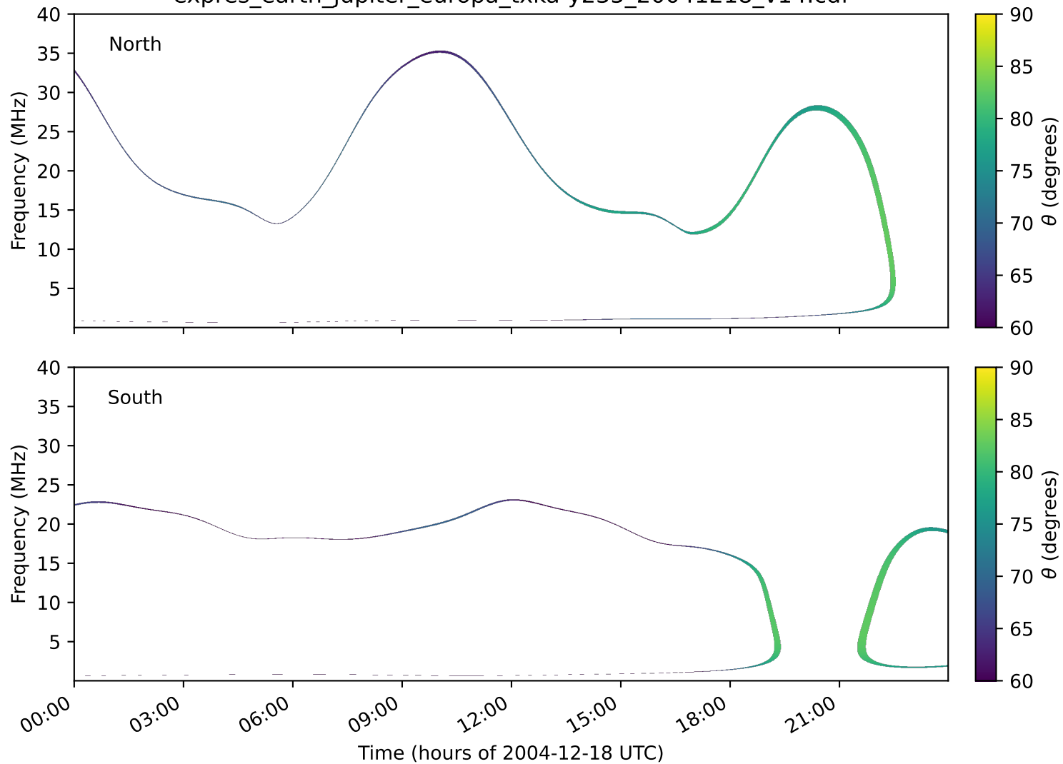
expres_earth_jupiter_europa_txka-y235_20041218_v14.cdf
