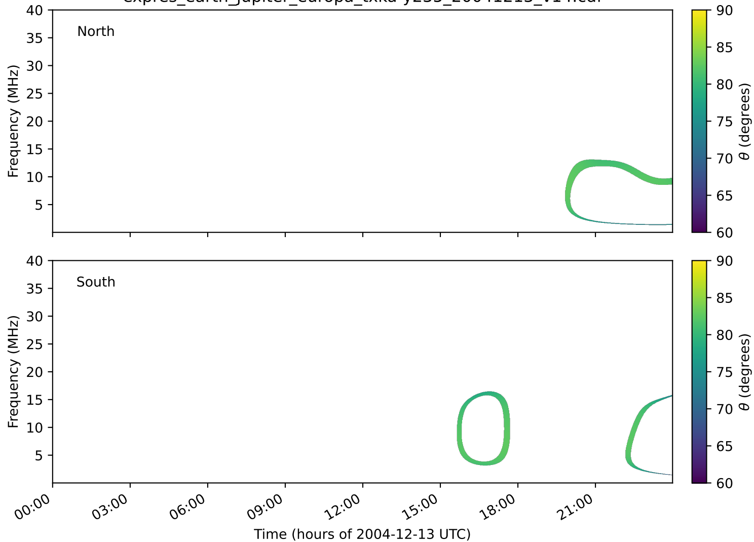
expres_earth_jupiter_europa_txka-y235_20041213_v14.cdf
