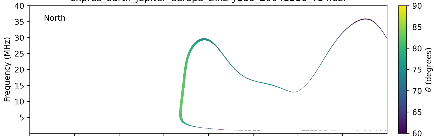
expres_earth_jupiter_europa_txka-y235_20041210_v14.cdf
