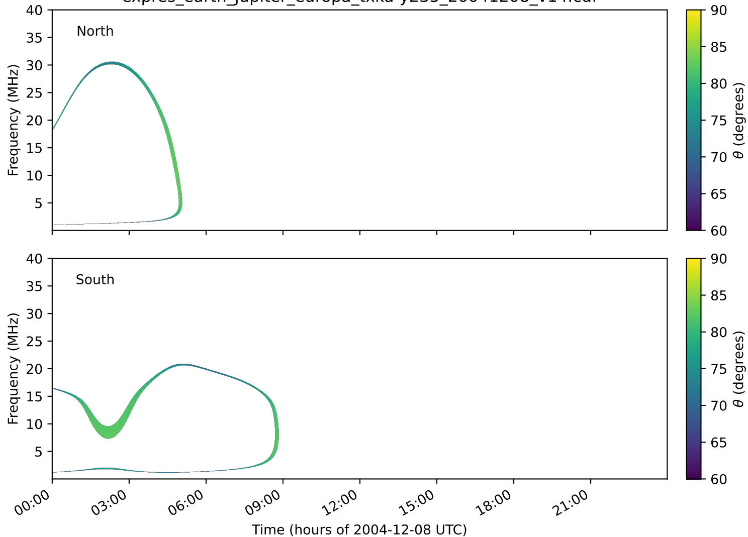
expres_earth_jupiter_europa_txka-y235_20041208_v14.cdf
