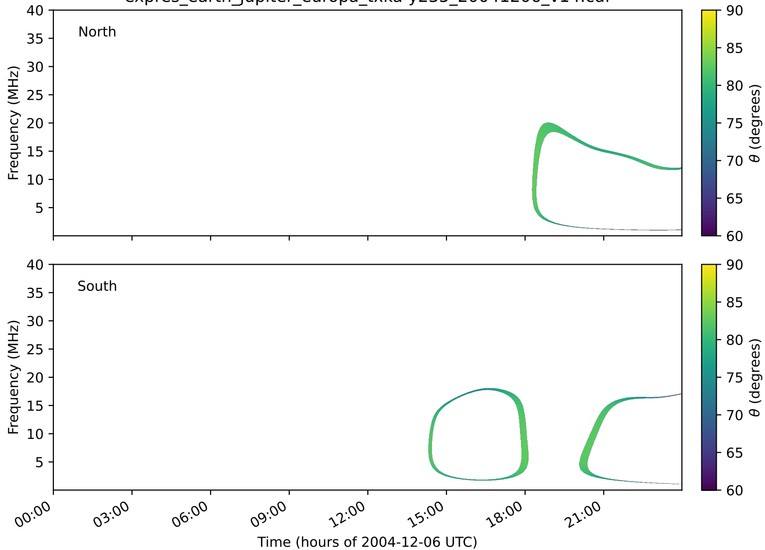
expres_earth_jupiter_europa_txka-y235_20041206_v14.cdf
