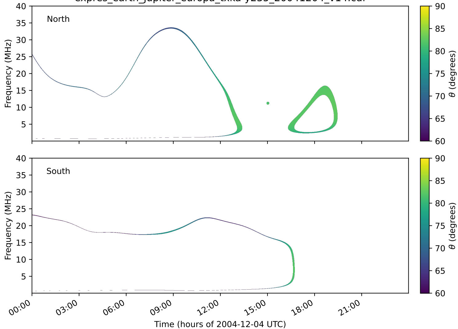
expres_earth_jupiter_europa_txka-y235_20041204_v14.cdf
