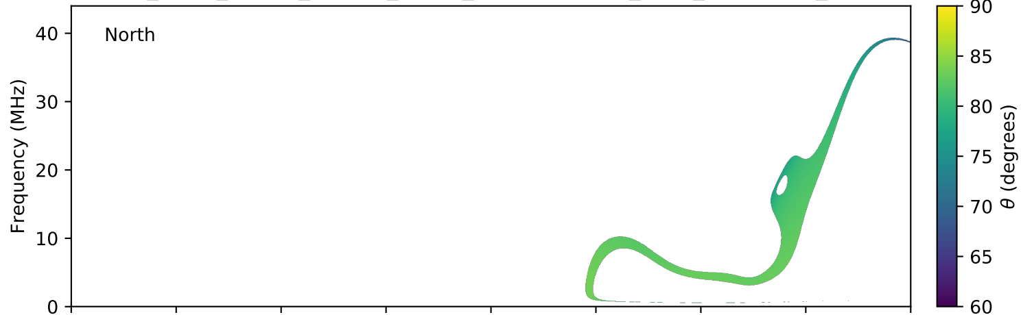
expres_earth_jupiter_europa_jrm09_lossc-wid1deg_3kev_20041231_v11.cdf
