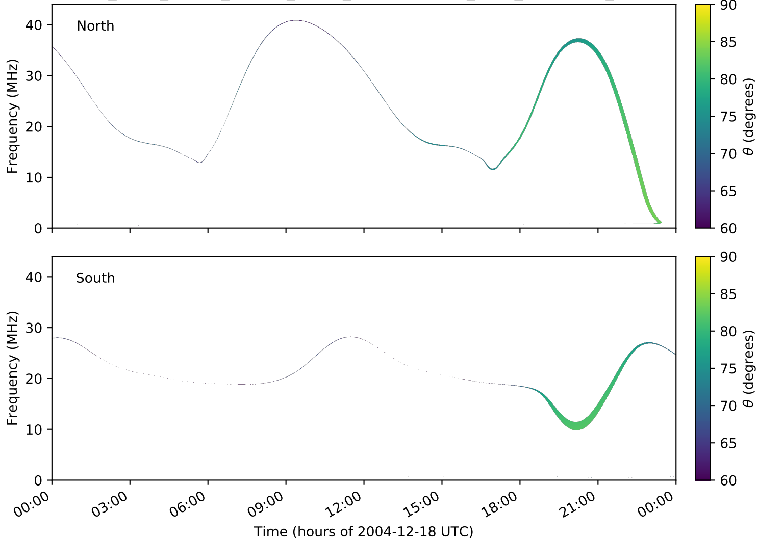
expres_earth_jupiter_europa_jrm09_lossc-wid1deg_3kev_20041218_v11.cdf
