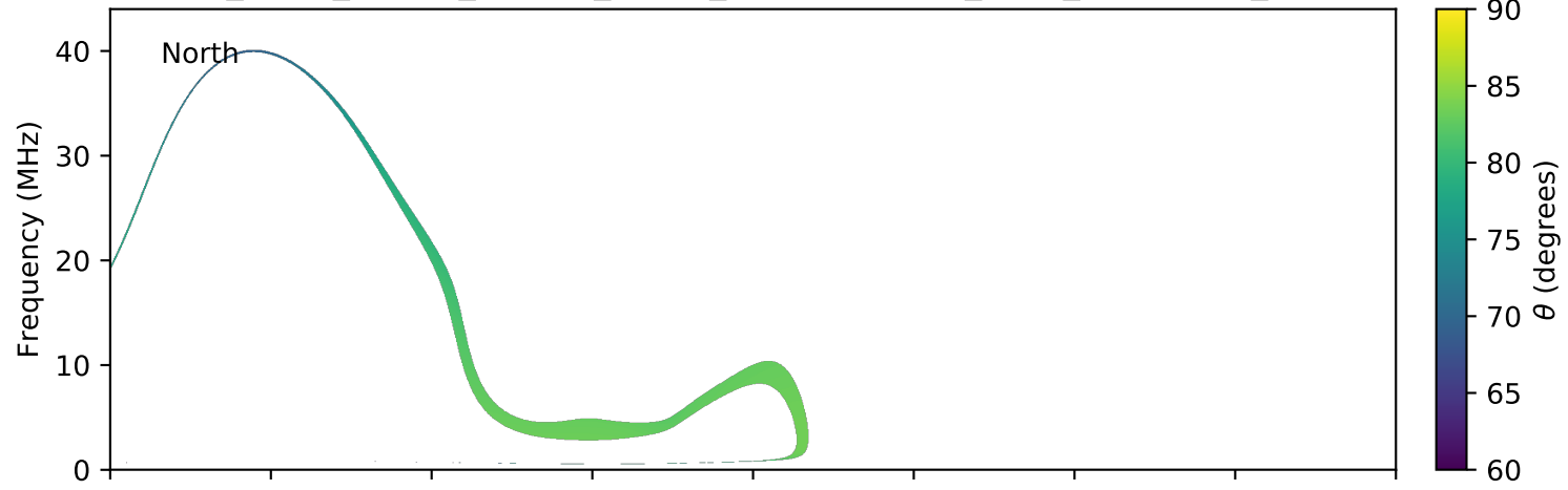
expres_earth_jupiter_europa_jrm09_lossc-wid1deg_3kev_20041215_v11.cdf
