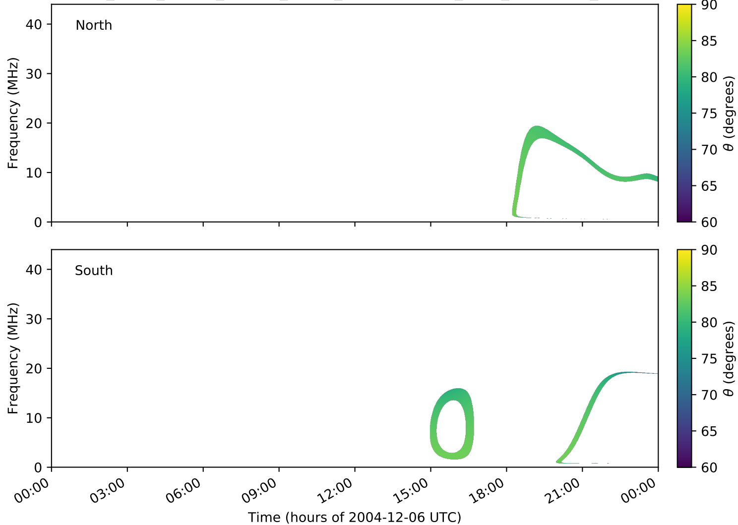
expres_earth_jupiter_europa_jrm09_lossc-wid1deg_3kev_20041206_v11.cdf
