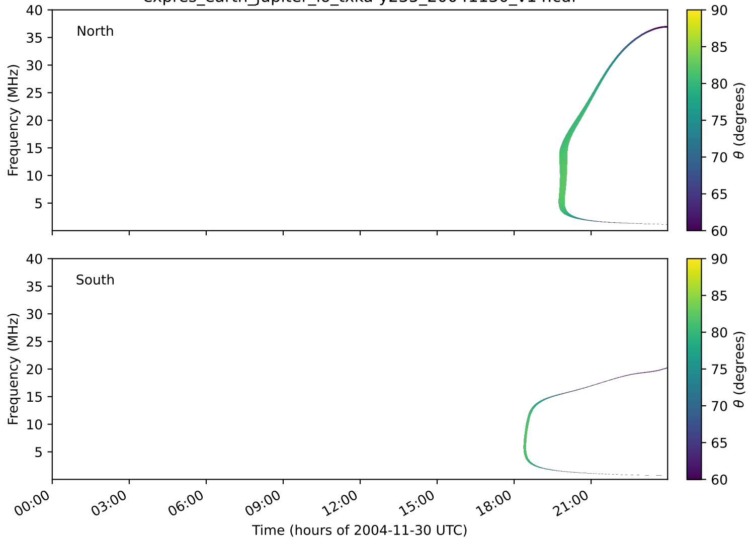
expres_earth_jupiter_io_txka-y235_20041130_v14.cdf
