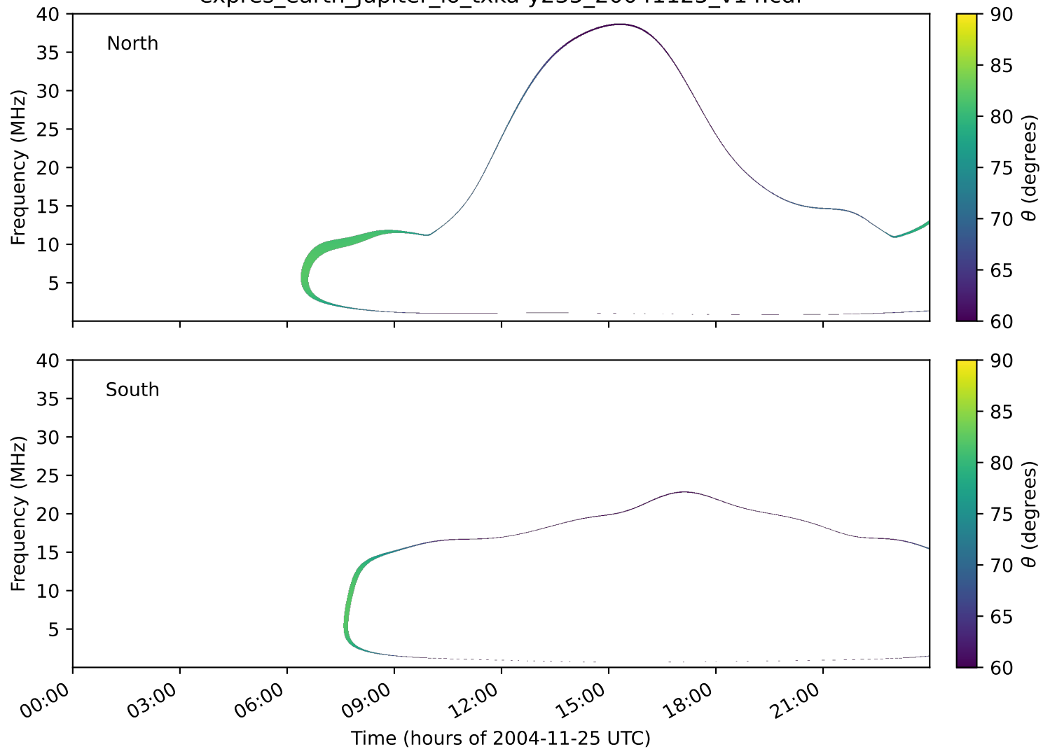
expres_earth_jupiter_io_txka-y235_20041125_v14.cdf
