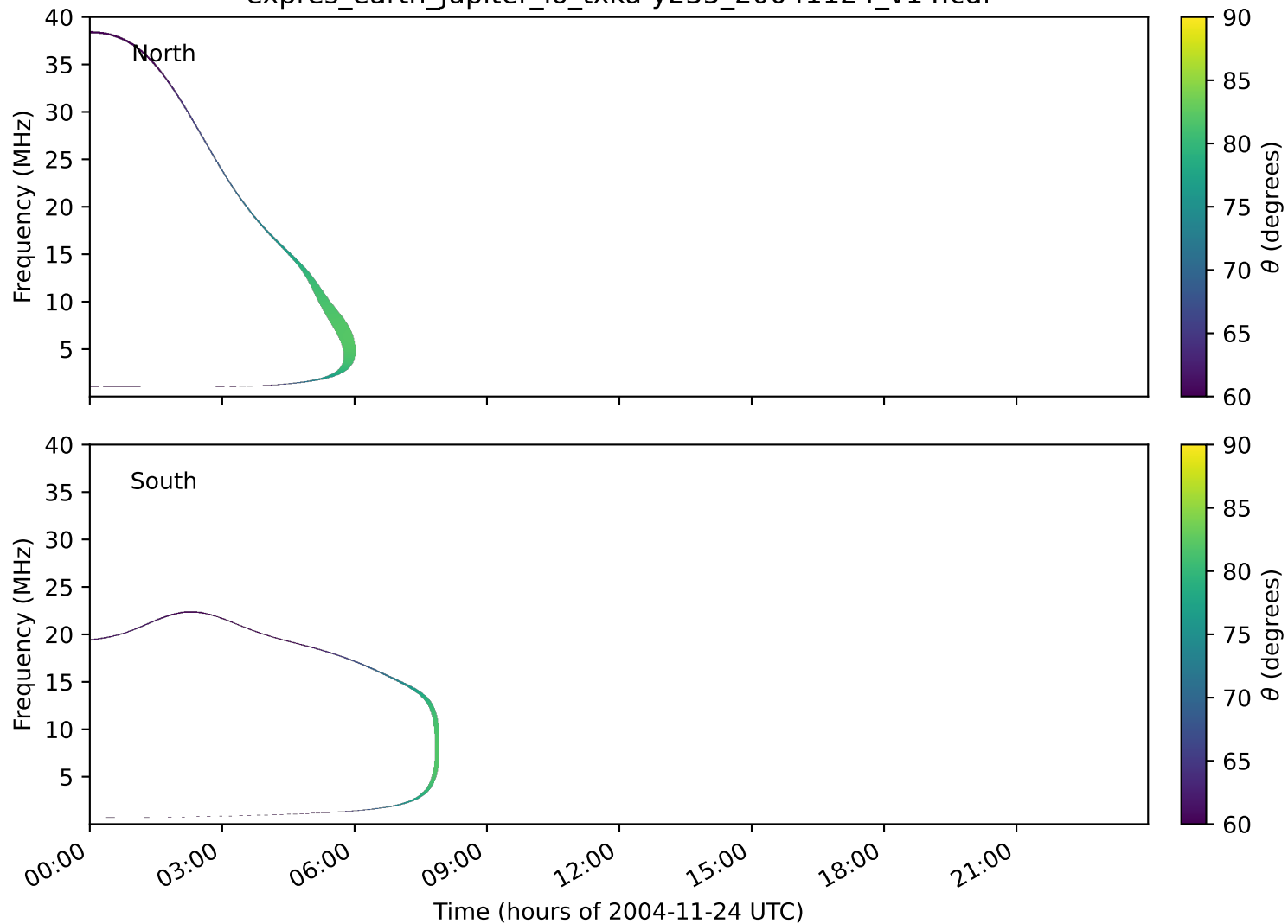
expres_earth_jupiter_io_txka-y235_20041124_v14.cdf
