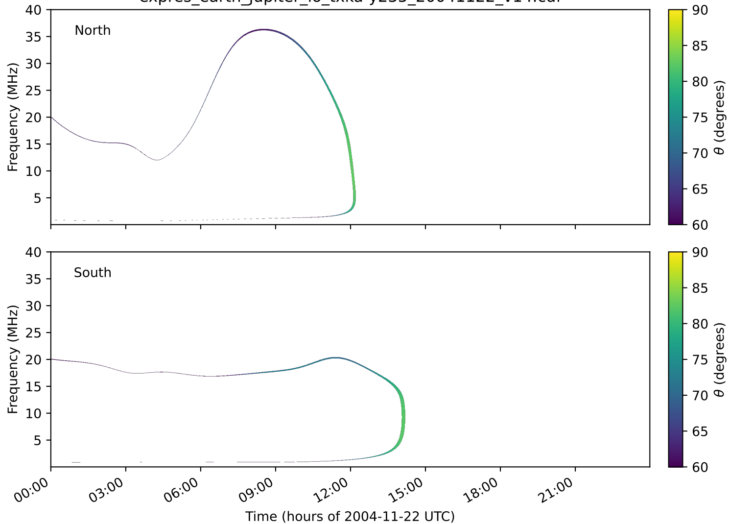
expres_earth_jupiter_io_txka-y235_20041122_v14.cdf
