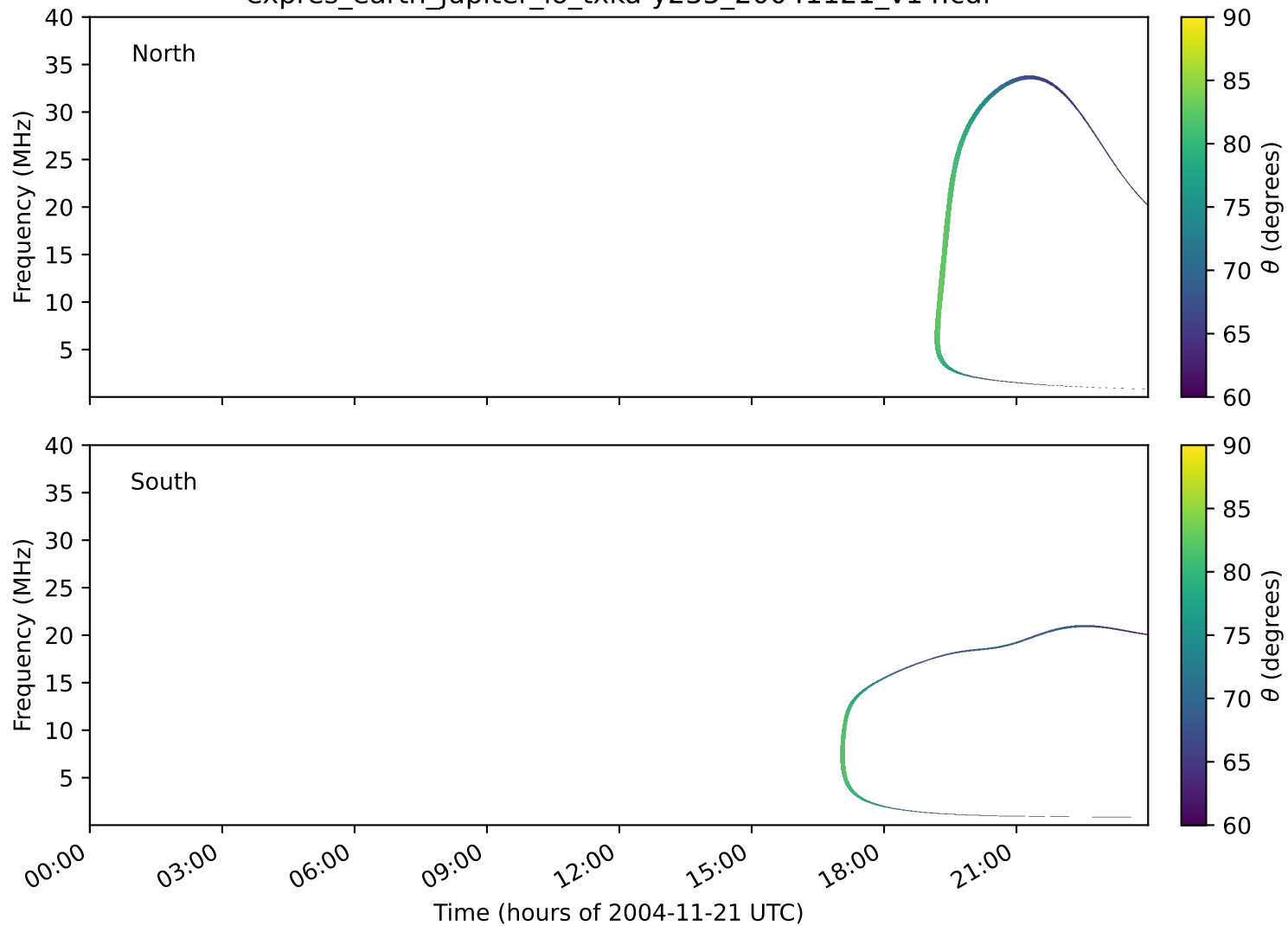
expres_earth_jupiter_io_txka-y235_20041121_v14.cdf
