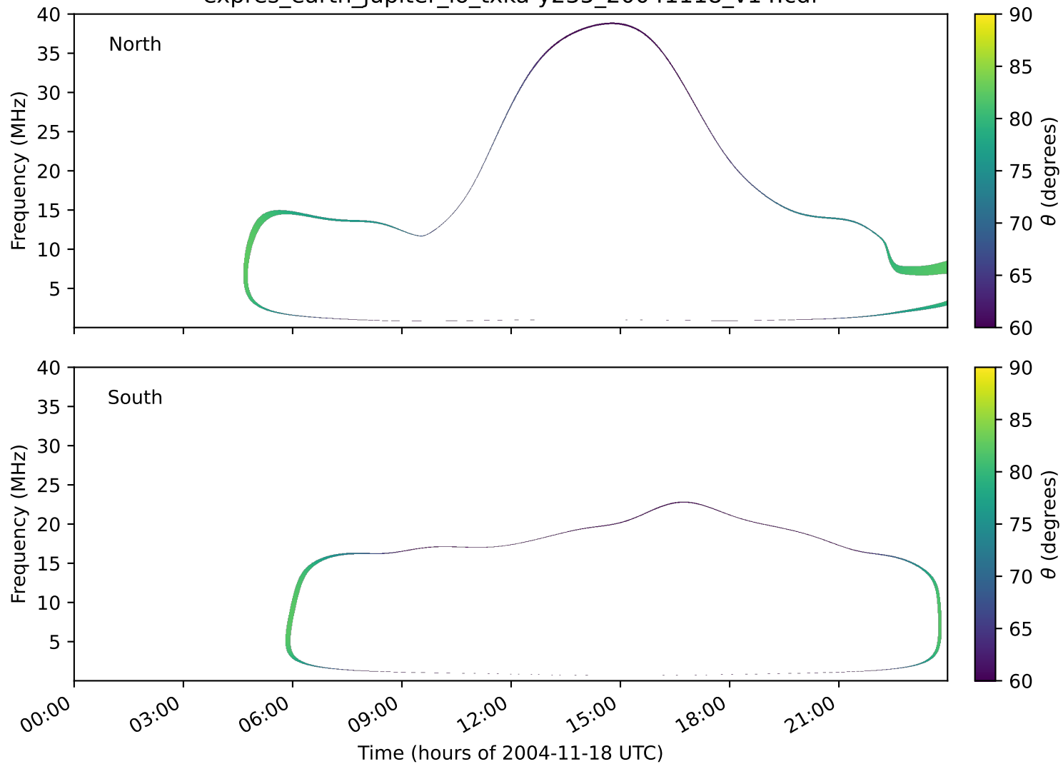
expres_earth_jupiter_io_txka-y235_20041118_v14.cdf
