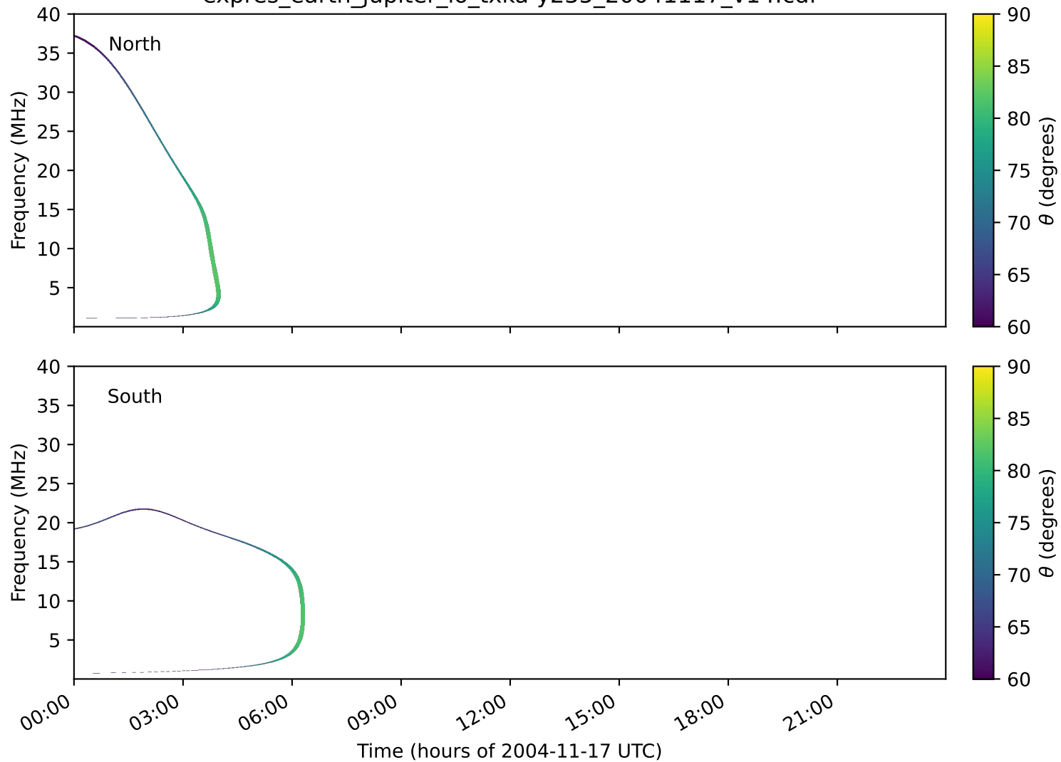
expres_earth_jupiter_io_txka-y235_20041117_v14.cdf
