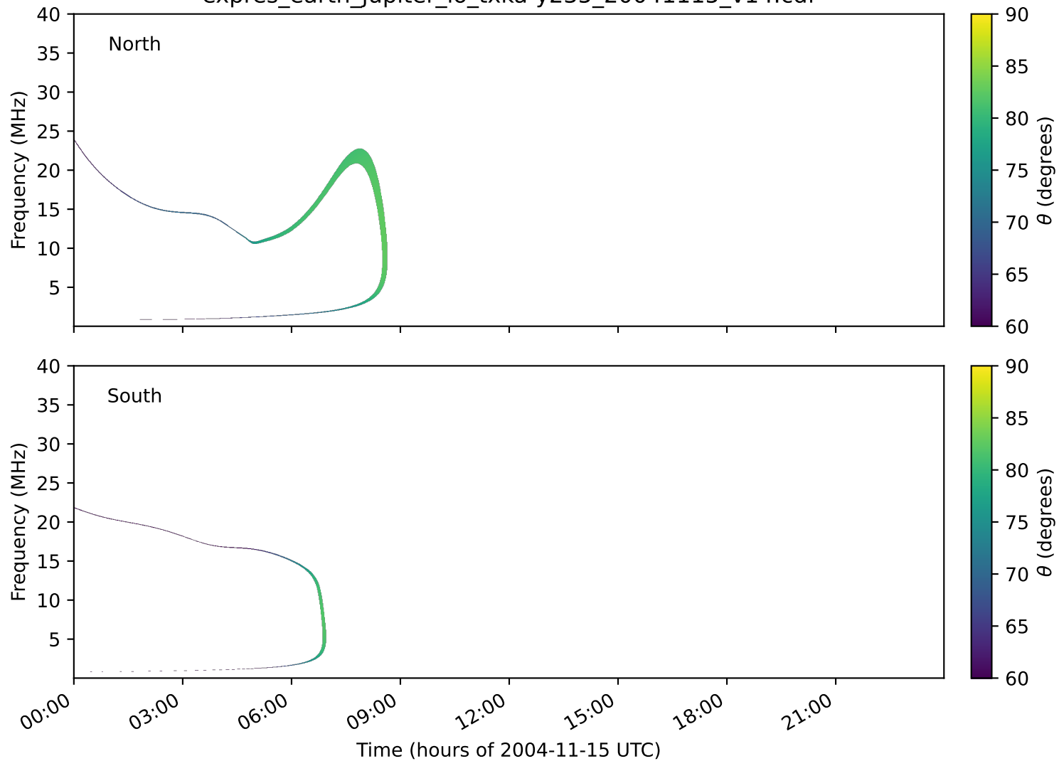
expres_earth_jupiter_io_txka-y235_20041115_v14.cdf
