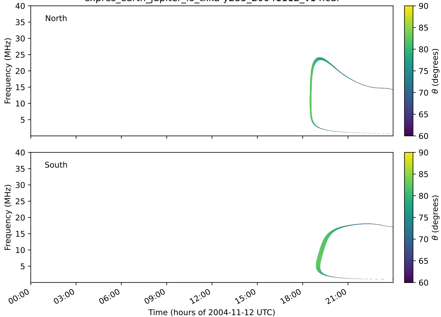
expres_earth_jupiter_io_txka-y235_20041112_v14.cdf
