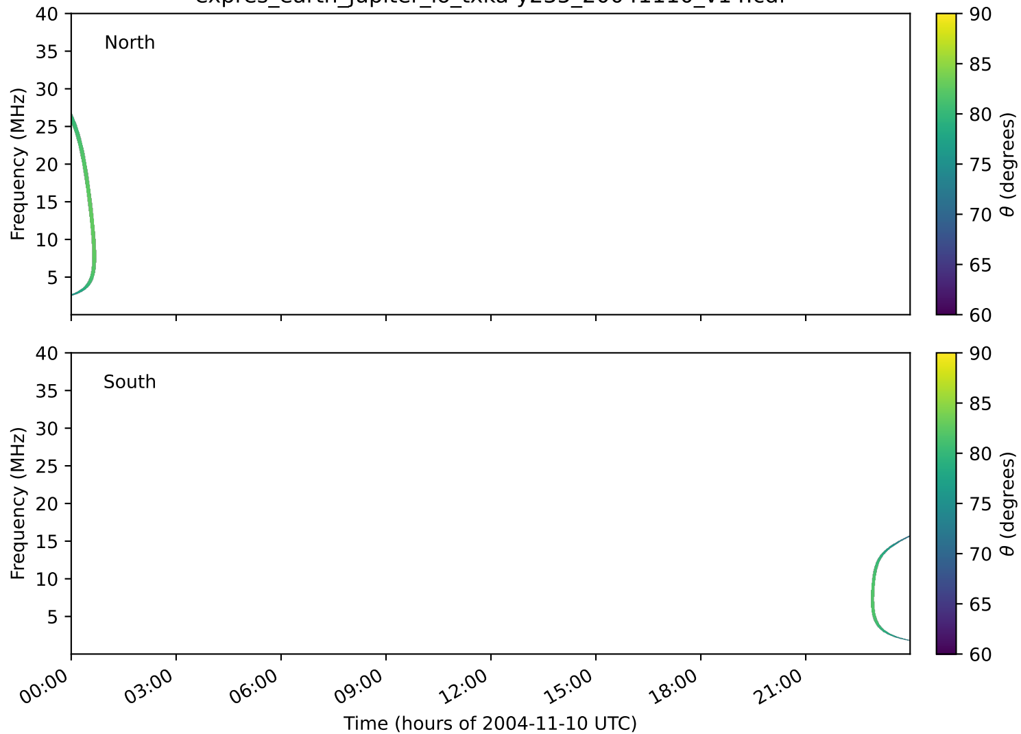
expres_earth_jupiter_io_txka-y235_20041110_v14.cdf
