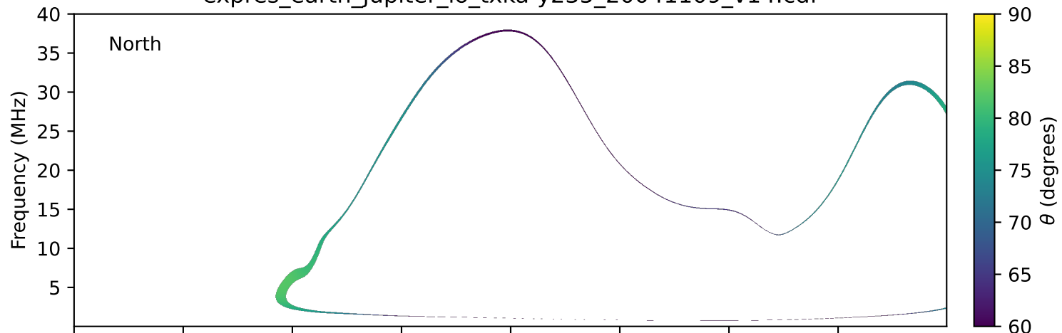
expres_earth_jupiter_io_txka-y235_20041109_v14.cdf
