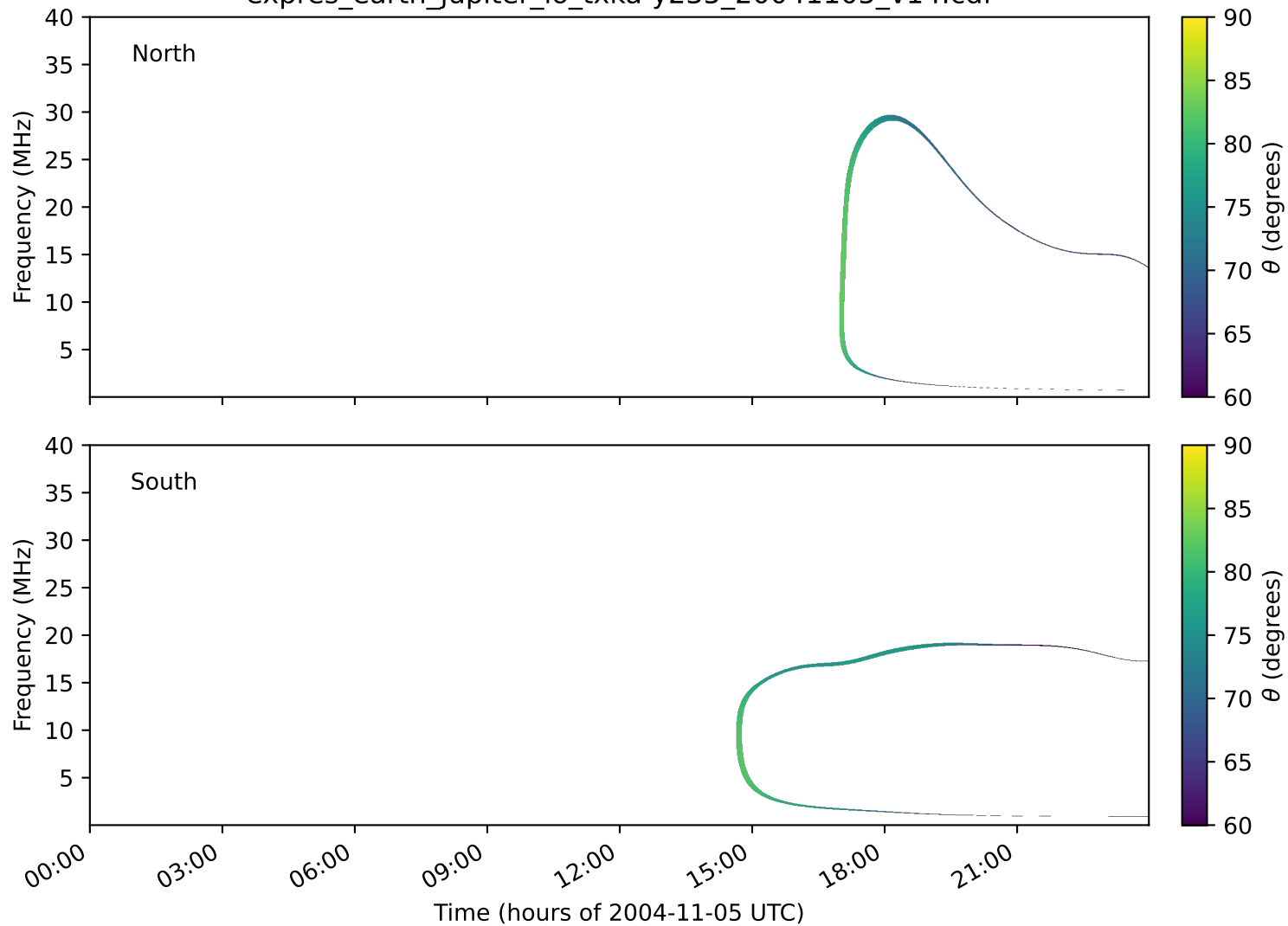
expres_earth_jupiter_io_txka-y235_20041105_v14.cdf
