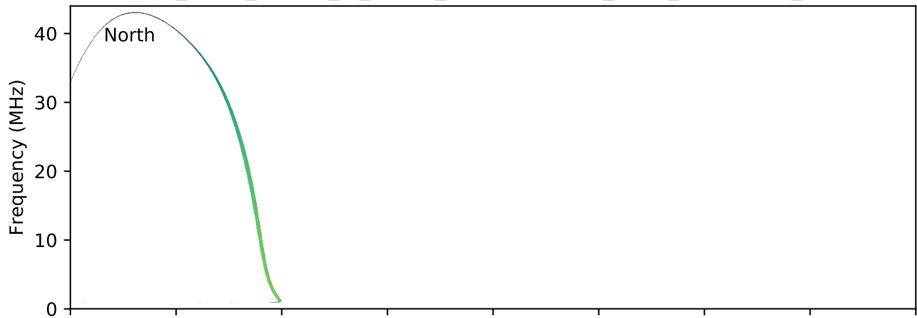
expres_earth_jupiter_io_jrm09_lossc-wid1deg_3kev_20041126_v11.cdf
