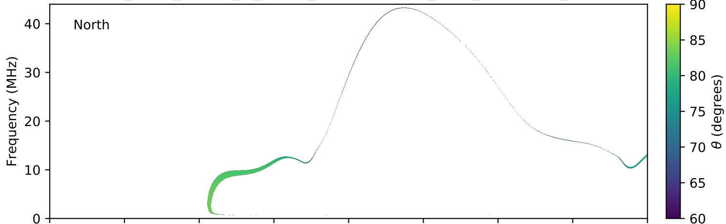
expres_earth_jupiter_io_jrm09_lossc-wid1deg_3kev_20041125_v11.cdf
