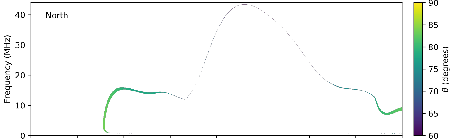
expres_earth_jupiter_io_jrm09_lossc-wid1deg_3kev_20041118_v11.cdf
