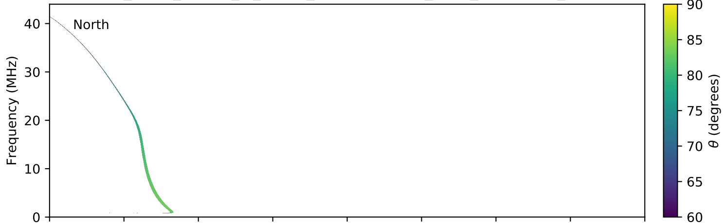
expres_earth_jupiter_io_jrm09_lossc-wid1deg_3kev_20041117_v11.cdf
