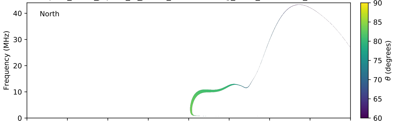
expres_earth_jupiter_io_jrm09_lossc-wid1deg_3kev_20041114_v11.cdf
