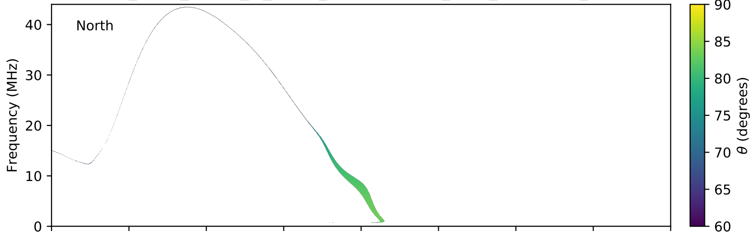
expres_earth_jupiter_io_jrm09_lossc-wid1deg_3kev_20041113_v11.cdf
