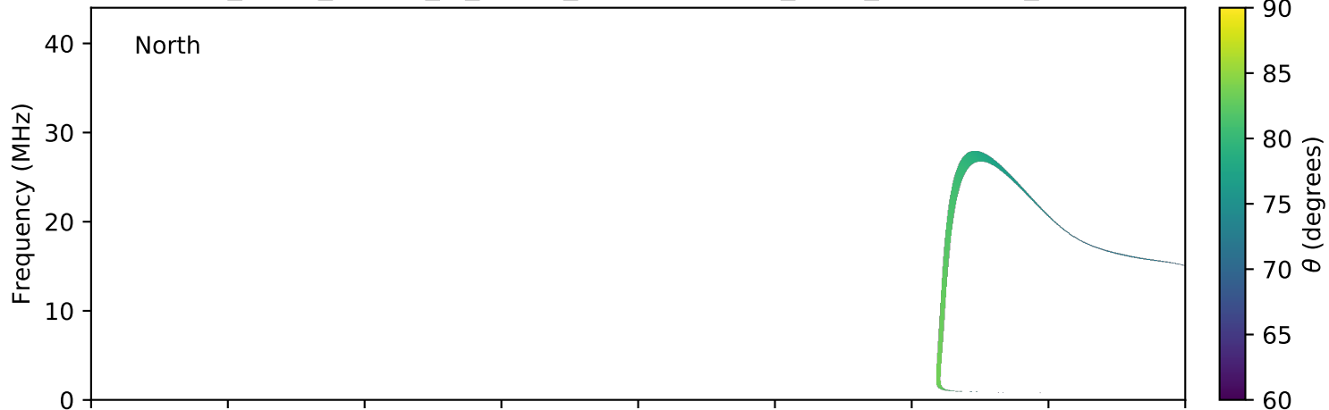
expres_earth_jupiter_io_jrm09_lossc-wid1deg_3kev_20041112_v11.cdf
